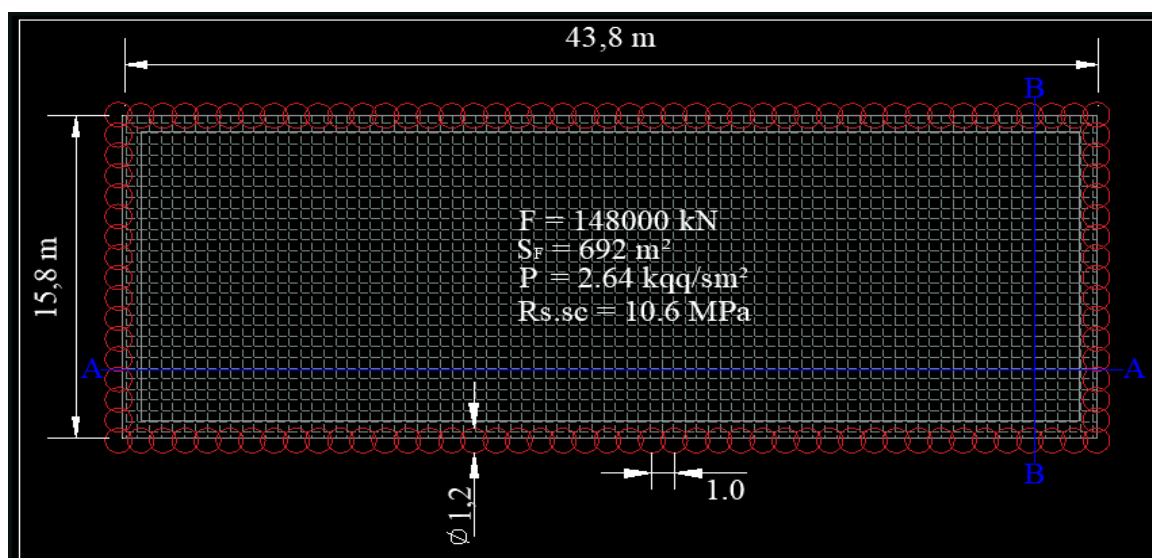
Figure 5 Scheme of application of Jet Grouting technology for protection of underground part of the building from groundwater
